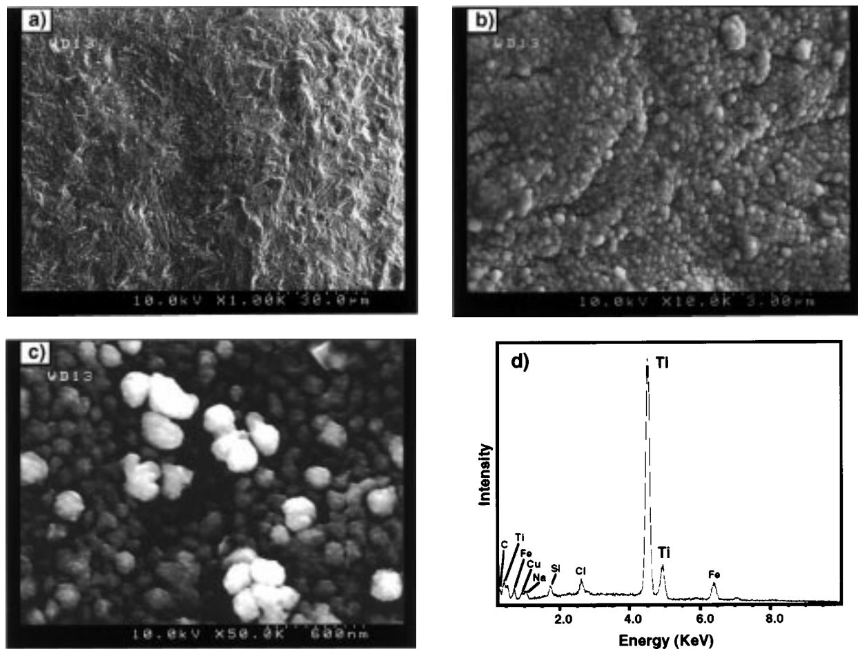
Figure 7. SEM images of sample R26 (grown on OFHC copper substrate at 610 °C) taken at (a) image magnification of 1000; (b) image magnification of 10 000; (c) image magnification of 50 000; (d) EDS spectrum of film shows clearly the presence of titanium, trace signals of Cu, Na, Si, Cl and Fe, and no oxygen signal. 23 The Cu signal is from the substrate and the weakness of the signal is due to the titanium overlayer. An EDS beam energy of 10 keV was used.
