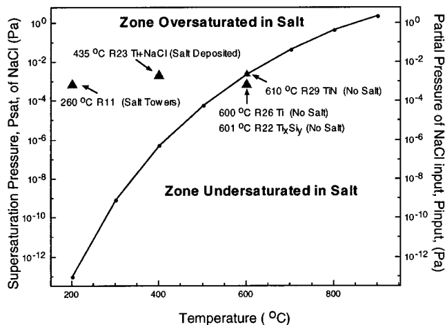
Figure 5. Plot of the supersaturation pressure of NaCl in the reaction zone ( P_{\text{sat}} ) (left-hand axis) versus temperature and the plot the partial pressure of salt input ( P_{\text{input}} ) (right-hand axis) versus temperature. The area above the solid curve should be oversaturated in salt (salt will deposit on the film), while area under the curve will be undersaturated in salt (salt will not deposit on the film). The solid curve was determined from thermodynamics calculations 14 and the triangles are individual experimentally determined points from the reaction conditions (substrate temperature and \text{TiCl}_4 input into the reaction zone).
