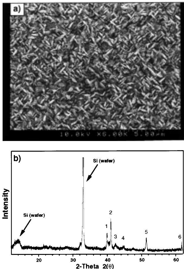
Figure 6. (a) SEM image of sample R22 grown on Si(100) at 600 °C showing two preferred growth orientations orthogonal to each other. (b) XRD spectrum of sample showing that titanium silicides ( Ti_xSi_y ) have formed. At 600 °C, the deposited Ti reacted with the silicon substrate to form titanium silicides, as has been previously reported in the literature. 20 See Table 2 for identification of the numbered peaks.
