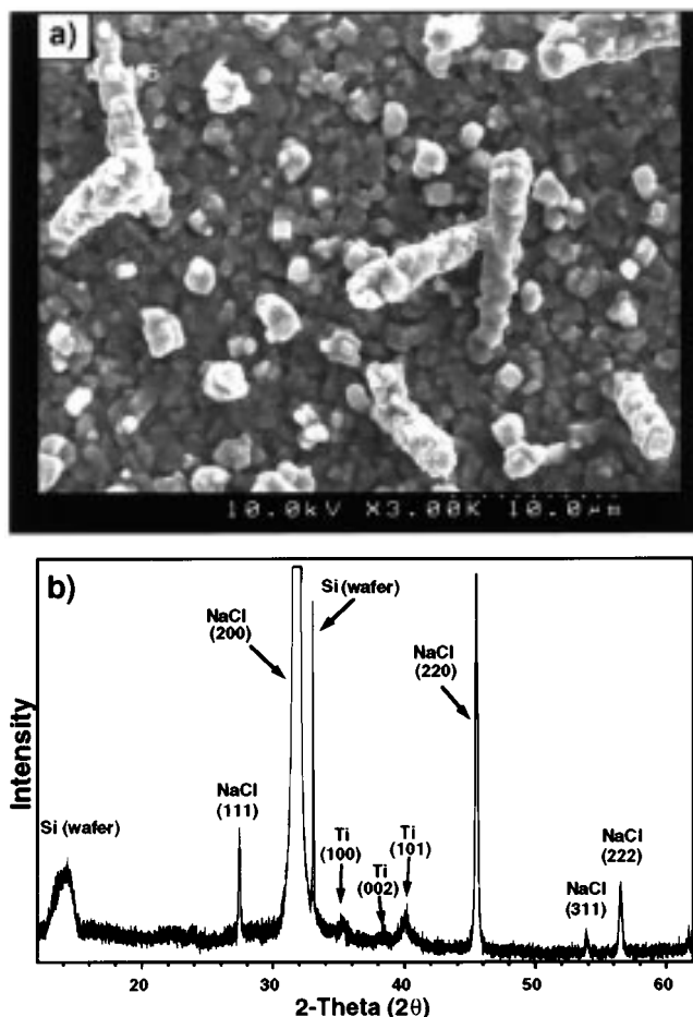
Figure 2. (a) Scanning electron microscope (SEM) of sample R23 (see Table 1 for reactor conditions). A 435 °C Si(100) substrate was used for the deposition surface. This image shows NaCl + Ti deposits. The tall columnar structures are likely to be salt, and their size and shape indicates a surface growth mechanism. (b) X-ray diffraction (XRD) spectrum of sample R23 showing the presence of both NaCl and Ti metal.
