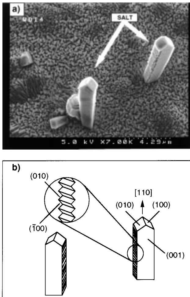
Figure 3. (a) SEM image of sample R11 (see Table 1 for reactor conditions). A 260 °C Si(100) substrate was used for the deposition surface. The tall towers are pillars of NaCl. The lower substrate temperature has increased the amount of salt deposited on the substrate surface. XRD analysis of this film confirmed the overwhelming presence of salt (NaCl). (b) Schematic representation of salt "towers". The edge of the salt tower shows that faceted crystal growth has occurred along the (100) planes. The tower shape appears to be due to rapid growth along the [110] direction orthogonal to the substrate surface.
