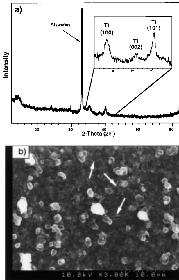
Figure 4. (a) XRD spectrum of sample R23W (the film remaining on the Si(100) substrate after rinsing sample R23 with water). X-ray analysis shows clearly the presence of titanium (see inset). All previously detectable salt peaks (see Figure 2b) are no longer present. (b) SEM image of sample R23W showing that the columnar structures shown in Figure 2a are now absent (further evidence that the columnar structures were primarily composed of NaCl). Note that cracking of the film is evident and is probably caused by film stress due to dissolving of salt from the film matrix.
