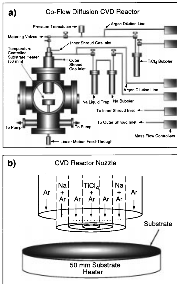
Figure 1. (a) Schematic of the low-pressure coflow diffusion CVD reactor used to react alkali metal vapor with metal halide vapor to deposit metal and ceramic films. Typical reactor conditions are listed in Table 1. (b) Schematic of the reactor nozzle consisting four concentric stainless steel tubes having dimensions of (i.d./o.d.) 5.38 mm/6.35 mm, 14.22 mm/15.88 mm, 24.13 mm/25.15 mm, and 36.07 mm/37.95 mm. The injection of reactants is as shown above.
