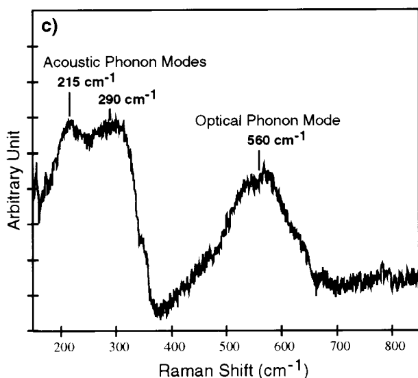
Figure 8. SEM images of sample R29 deposited on a OFHC copper substrate at 610 °C showing (a) image magnification of 10 000 and (b) image magnification of 100 000. Figure 8b shows clearly that the film consists of cubic crystallites with an edge length of ~60 nm. (c) Raman spectrum of sample R29 showing that the deposited material is titanium nitride. The peaks at 215 and 290 \text{cm}^{-1} correspond to the acoustic phonon modes of TiN previously measured to be 200 and 280 \text{cm}^{-1} respectively. 24 The peak at 560 \text{cm}^{-1} corresponds to the optical phonon mode of TiN previously measured to be 520–550 \text{cm}^{-1} . 24
